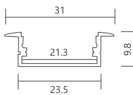
519-25X10MM COLLAR
