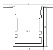
526(A)-8X6MM COLLAR
