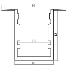
524(A)-10X13MM COLLAR
