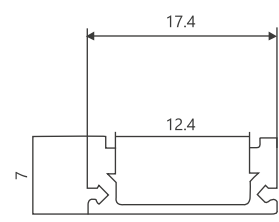
409-17X7MM COLLARLESS
