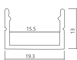
516-19X13MM COLLARLESS
