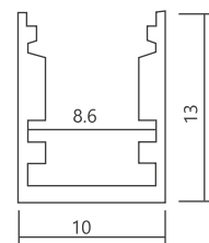
524-10X13MM COLLARLESS
