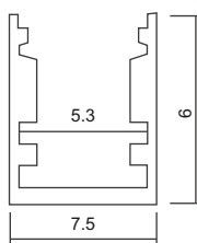
526-8X6MM COLLARLESS
