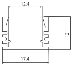
405-17X12MM COLLARLESS
