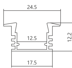
505-17X12MM COLLAR
