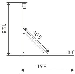
501-CORNER 16X16MM
