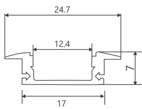
408-17X7MM COLLAR
