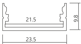
517-25X10MM COLLARLESS
